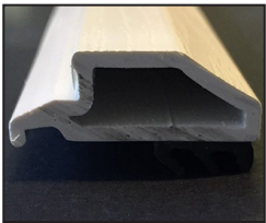
Flush Triple Glazing 32mm
